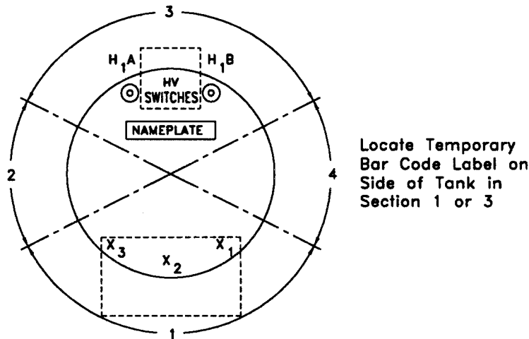
Figure 7—Temporary bar code label location on single-phase subsurface transformers
