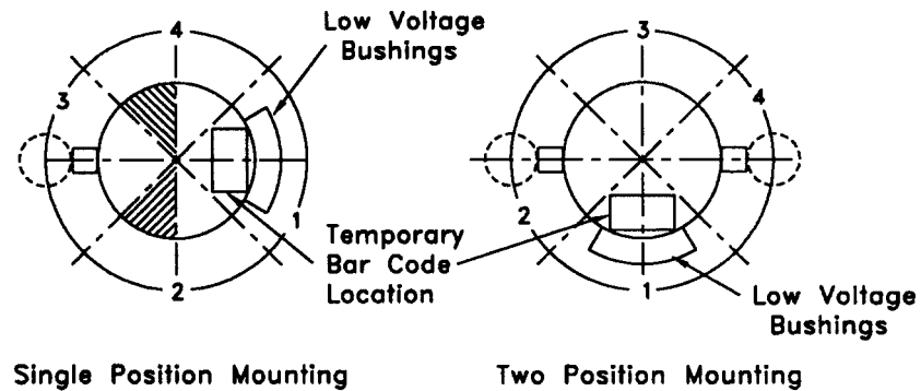
Figure 3—Temporary bar code location on overhead type distribution transformers single-phase, 50 kVA and below
