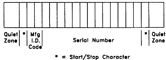
Figure 2—Data format, temporary label
