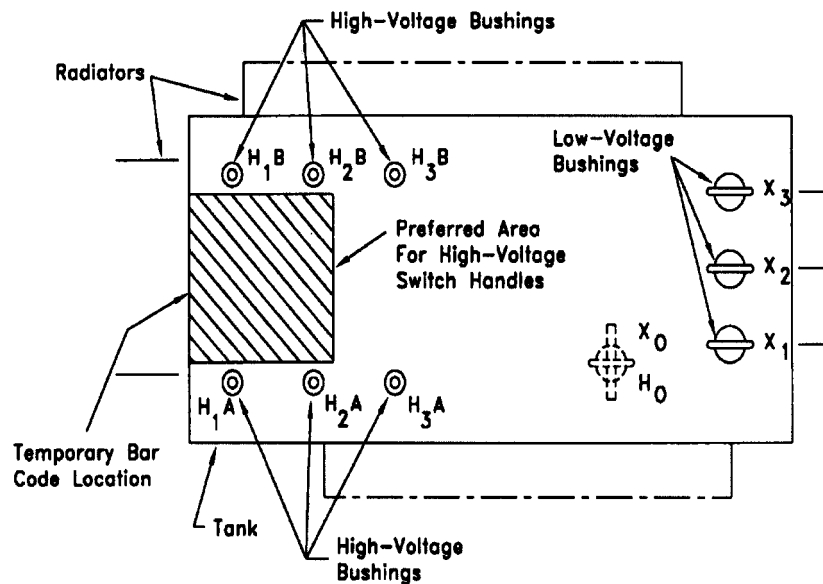
Figure 8—Temporary bar code label location on three-phase and network-type subsurface transformers
